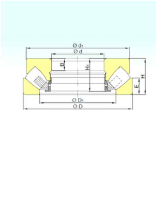
294/560 M Bearing 2D drawings and 3D CAD models
