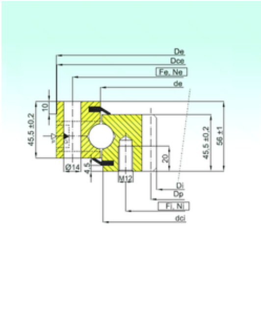
ZB1.20.0414.201-2SPTN Bearing 2D drawings and 3D CAD models
